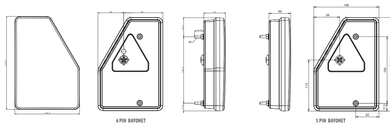
6 PIN BAYONET
