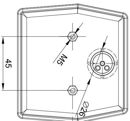
bayonet connection view
